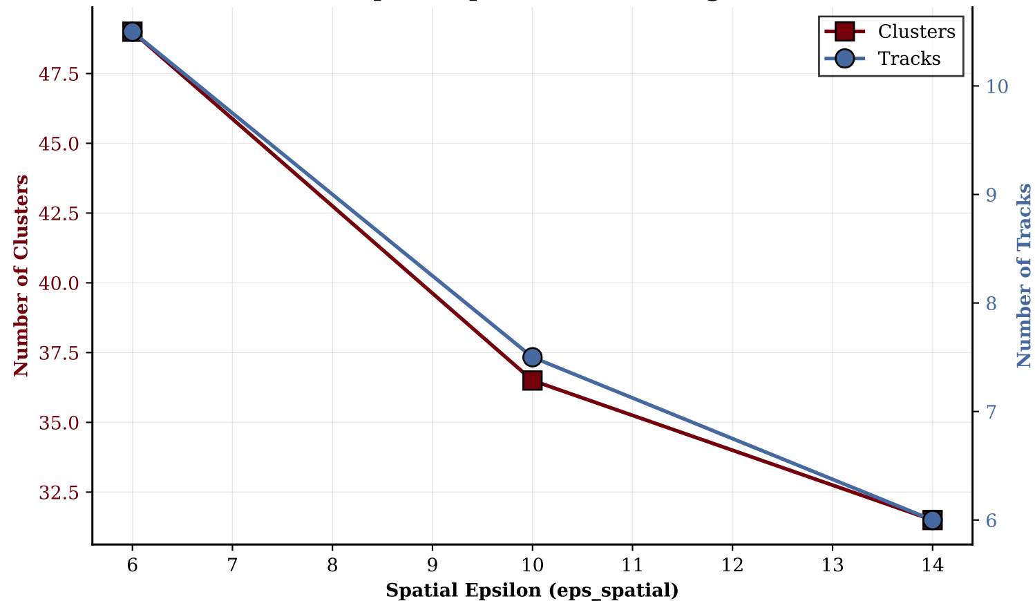
Effect of Spatial Epsilon on Clustering Results
